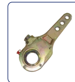
SLACK ADJUSTER KFD No.: KFD86011 OEM No.: KN44042 Specification: 3 HOLE 37 TEETH 5", 6", 7"
